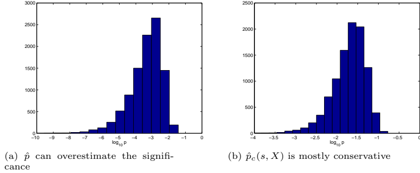
Fig. 2: Comparing the estimators \hat{p} and \hat{p}_c(s, X) of p = 10^{-3}
