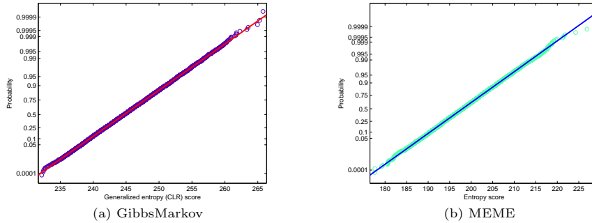
Fig. 1: Probability plots of 3-Gamma fits to the empirical score distribution
