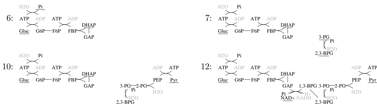
Figure 3: Expansion on the glycolytic pathway (case 3). Conditions, labels, and parameter values are the same as for Figure 2 with the exception that only water is considered to be highly abundant.
