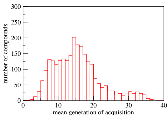
Figure 6: Histogram of mean generations of acquisition. Simulations have been performed for all compounds as explained for \text{NAD}^+ and glucose in the legend of Figure 5. The diagram includes the values of those compounds which were acquired in at least 5% of the simulations.
